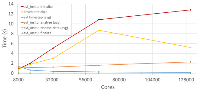
Fig. 15: AVF-LESLIE Performance with SENSEI/Libsim In Situ Processing 1025 3 Dataset (Render Session for Isosurface and Coordinate Cuts).
