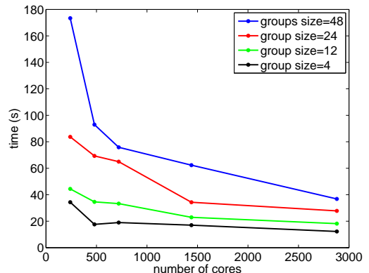
Figure 11: Query performance for different group sizes.
