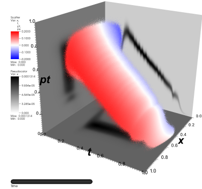
Figure 13: Scatter plot of all particles in x, t, pt space with particle color indicating the momentum in x direction p_x (red=positive, blue=negative). The axes of the plot have been normalized for display purposes. The gray plots on the side and bottom show the two-dimensional particle density in x/t, x/pt and t/pt , respectively.
