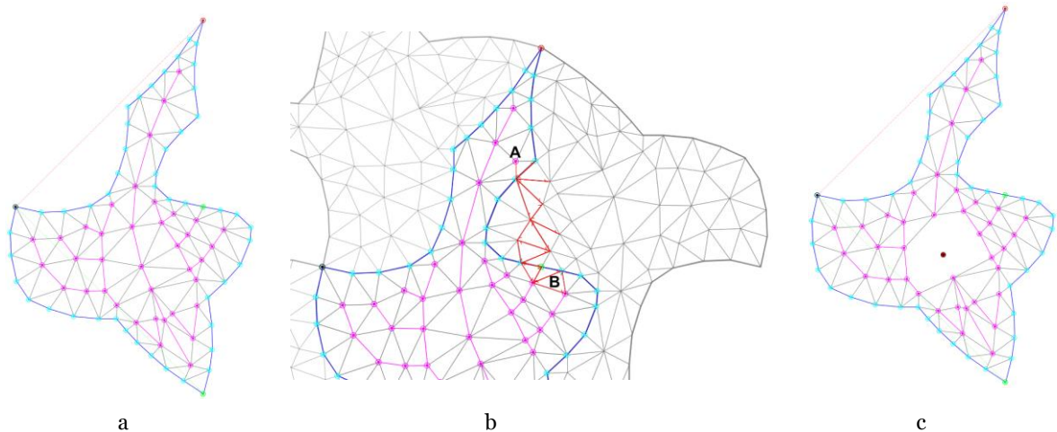
Fig. 5: Incremental Delaunay triangulation: (a) the mesh of a decorated fish tile with constrained edges (magenta); (b) a mesh search from vertex A to face B , which exploits the symmetry of the tile by moving directly through an adjacent copy; (c) the n -gonal hole resulting from removing a vertex.
