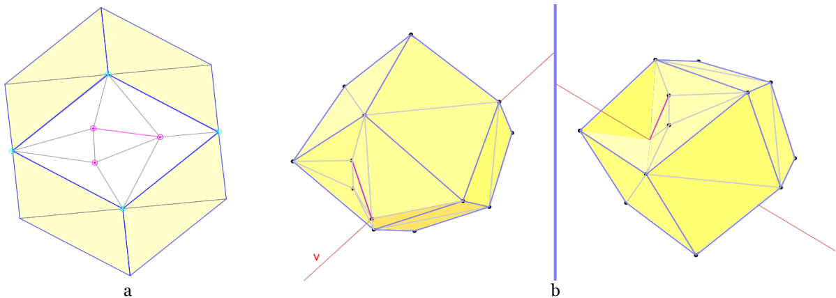
Fig. 8: Pane-based construction of a 3D Escher tile: (a) a pane of the dodecahedral tile available for 2D editing and Delaunay triangulation; and (b) free-form 3D vertex editing with dual cameras and a radial selection-and-extrusion vector v (red).
