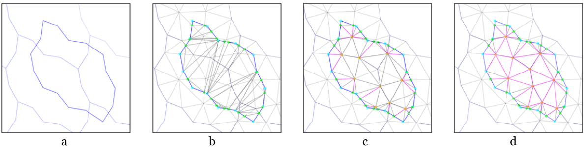
Fig. 6: Cookie-cutter operation: (a) a cookie-cutter contour (blue) has been offset from the underlying landscape (gray), whose meshes will subsequently be loaded on-demand; (b) intersection points (green) are found by walking the cookie-cutter boundary, which is temporarily filled with interior edges (gray) to enable later vertex insertions; (c) edge fragments in the active queue have been added as constraint edges (magenta); and (d) the remaining landscape edges lying inside the cookie cutter have been found via flood fill and added as constraint edges (magenta).
