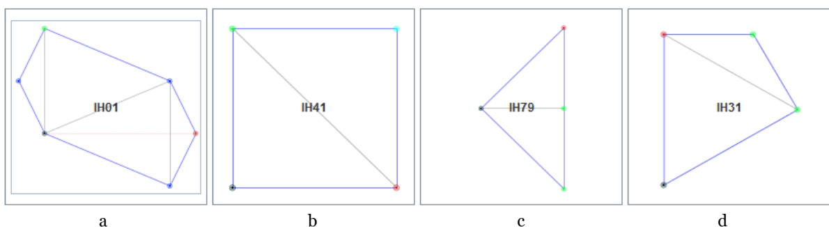
Fig. 2: Four 2D symmetry groups: (a) IH01, hexagonal domain with translational symmetry; (b) IH41, rectangular domain with translational symmetry; (c) IH79, right-triangle domain with 4-fold rotational symmetry; and (d) IH31, kite-shape domain with 6-fold rotational symmetry.
