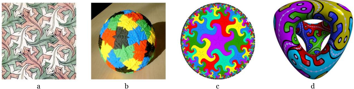
Fig. 1: Escher-like tilings on 2-manifolds: (a) in the plane; (b) on a sphere; (c) in the Poincaré disk; and (d) on a genus-3 "Tetrus" surface.
