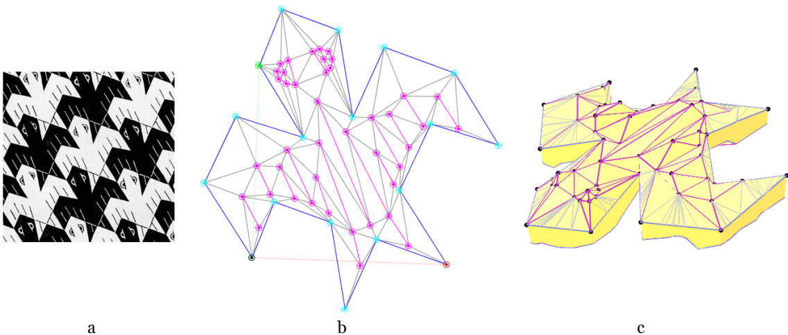
Fig. 10: A 2\frac{1}{2}D bird tile: (a) Escher’s sketch number 127 provides the basic contour; (b) interior vertices and constraint edges are added to provide control points for editing the height field; and (c) the edited height-field.
