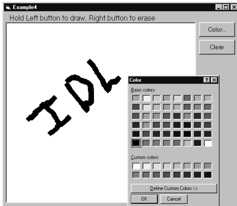
Figure 6-11: VBPaint example
