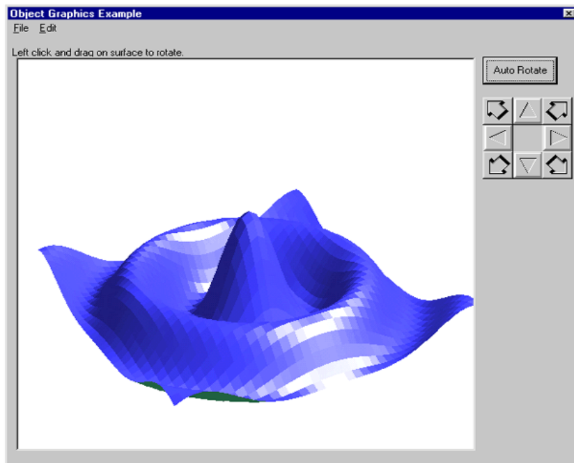
Figure 6-9: VBObjGraph example
