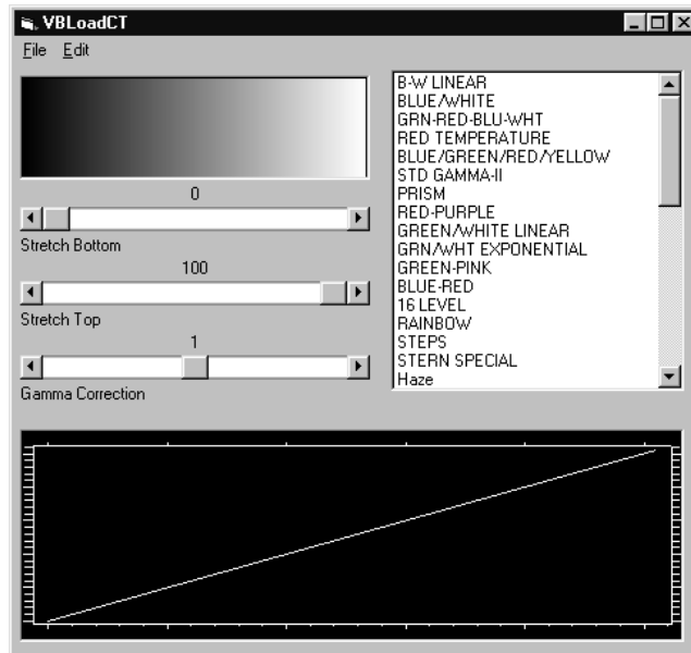
Figure 6-7: VBLoadCT example
