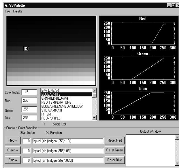
Figure 6-8: VBPalette Example
