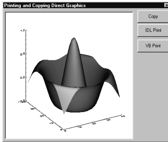
Figure 6-6: VBCopyPrint example
