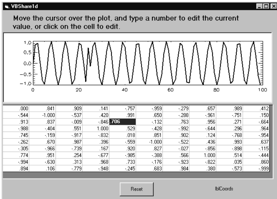
Figure 6-10: VBShare1D
