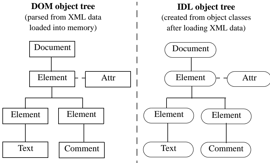
Figure 21-2: The DOM and IDL Trees
