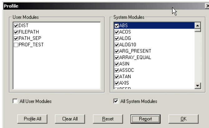
Figure 10-1: Profile Dialog
